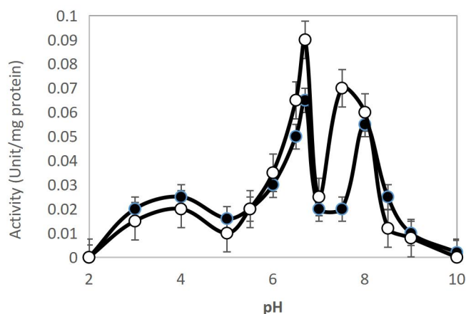
Figure 1: Determination of optimal pH for cresolase activity in Solanum lycopersicum under immature and mature conditions using p-cresol as the substrate.
