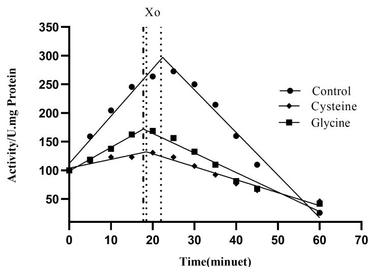
Figure 10: Effect of time on cresolase activity under immature conditions at the optimal temperature.
