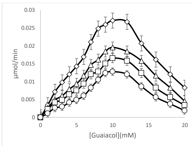
Figure 7: Determination of kinetic parameters of GPX activity in S. lycopersicum extract (ripe stage) in the presence of guaiacol. Absence of Cys ( \diamond ), 0.4 mM Cys ( \Delta ), 0.8 mM Cys ( \square ), 1.2 mM Cys ( \circ )
