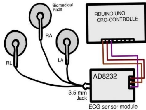
Figure 2: The connections between the Arduino Uno and the ECG sensor module, including the 3.5mm jack and the AD8232 chip.
