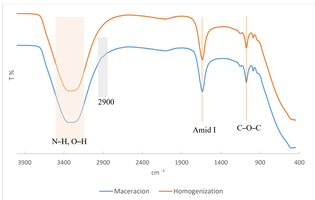
Fig 1. FTIR spectrum of the products from maceration and homogenization extract methods from Gelidium pusillum .
