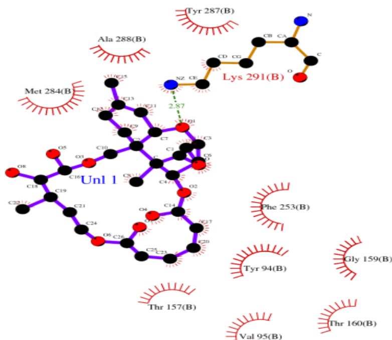
Figure 5: Docked conformation of Verrucarin A at the active site of ACC Oxidase (ACO) illustrating ligand-protein interactions
