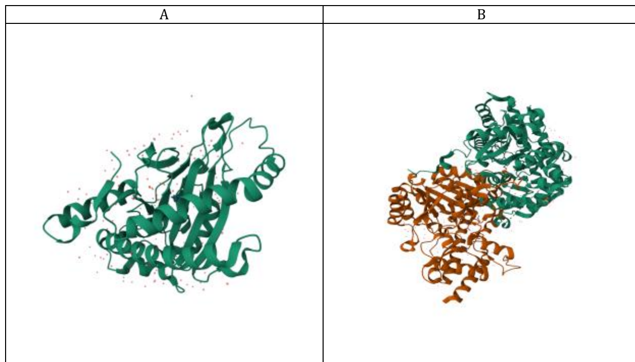
Figure 2. Three-dimensional structures of ACC Oxidase (A) and ACC Synthase (B) involved in the ethylene biosynthesis pathway
