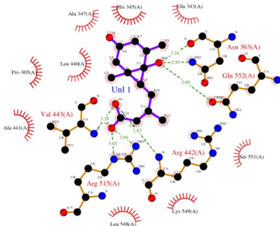
Figure 7: Docked conformation of Absciscic Acid at the active site of Isochorismate Synthase (ICS) illustrating ligand–protein interaction
