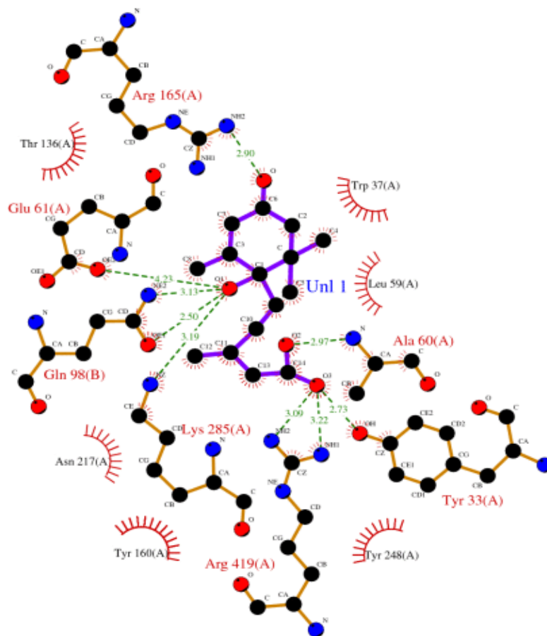
Figure 6: Docked conformation of Absciscic Acid at the active site of ACC Synthase (ACS) illustrating ligand–protein interaction
