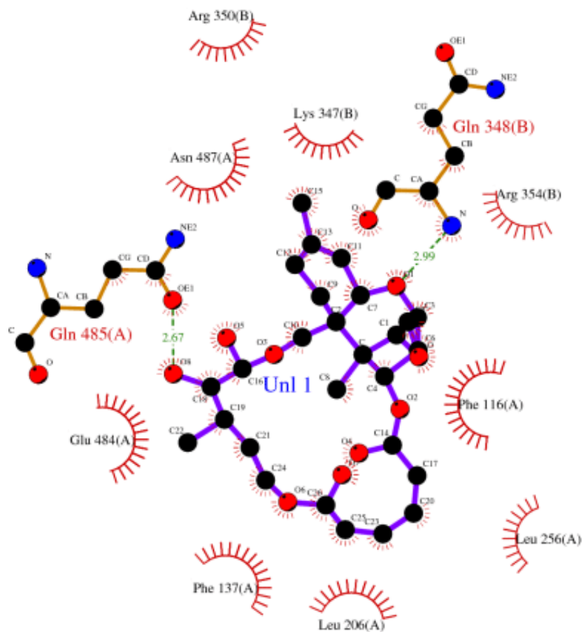
Figure 8: Docked conformation of Verrucaric acid at the active site of Phenylalanine Ammonia-Lyase (PAL) illustrating ligand–protein interaction
