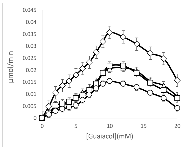
Figure 9: Determination of kinetic parameters of GPX activity in S. lycopersicum extract (ripe stage) in the presence of guaiacol. Absence of Cys (◇), 0.4 mM Cys (Δ), 0.8 mM Cys (□), 1.2 mM Cys (○)
