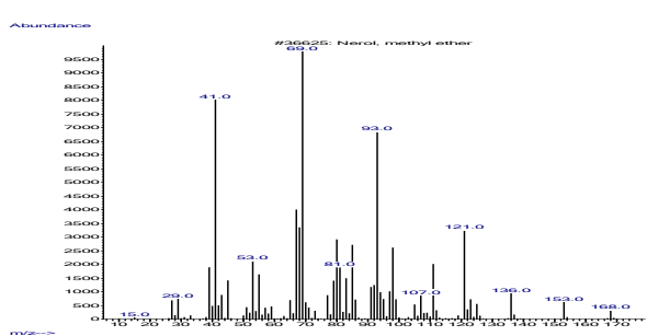
Fig. 6B: Mass spectra of Nerol, methyl ether
