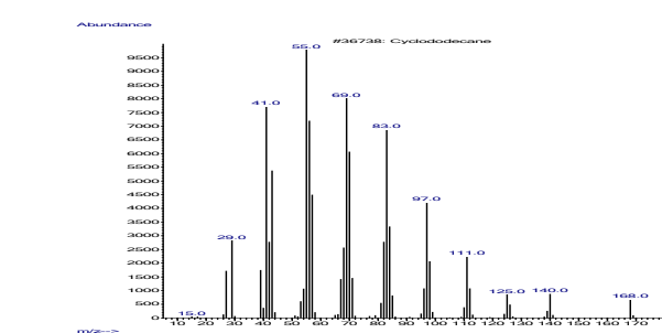
Fig. 6A: Mass spectra of Cyclododecane
